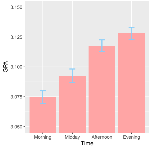
Figure 4: Simulated average grade if all courses were offered at the same time of day. Note that the y-axis does not start at 0. The 95% confidence intervals shown are basic bootstrap confidence intervals calculated using the distribution of student grades predicted by the model.
