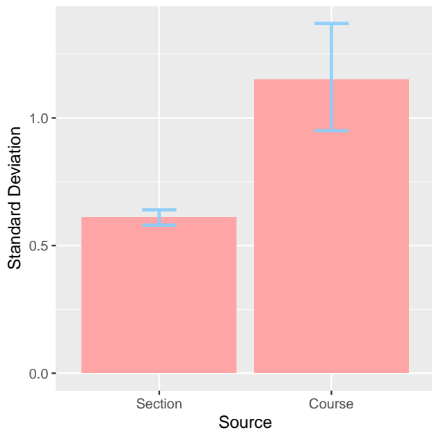
Figure 5: Standard deviation of the section level ( U_{jk} ) and course level ( W_k ) error terms from the model, with the 95% credible intervals provided by the Bayesian estimation.
