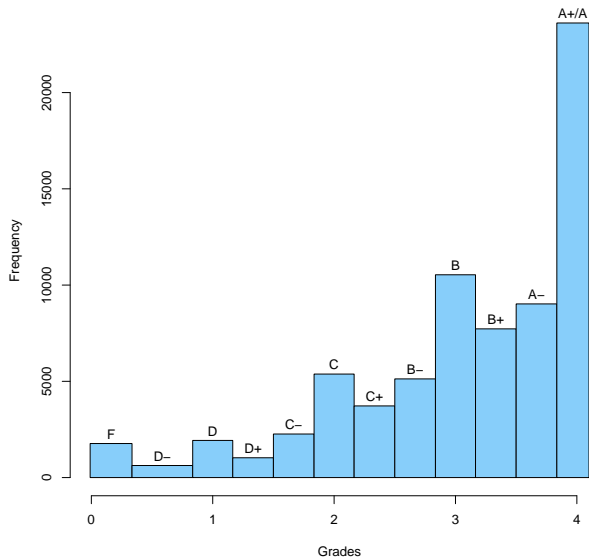
Figure 1: All student grades in the data set.
