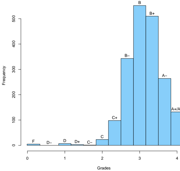
Figure 2: Distribution of section averages
