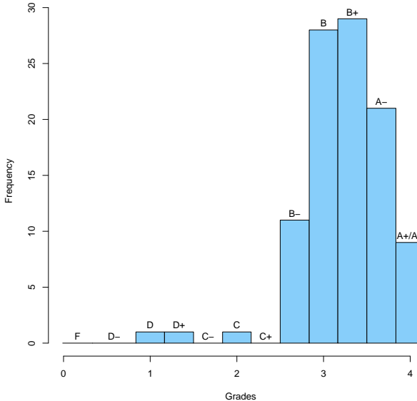
Figure 3: Distribution of course averages
